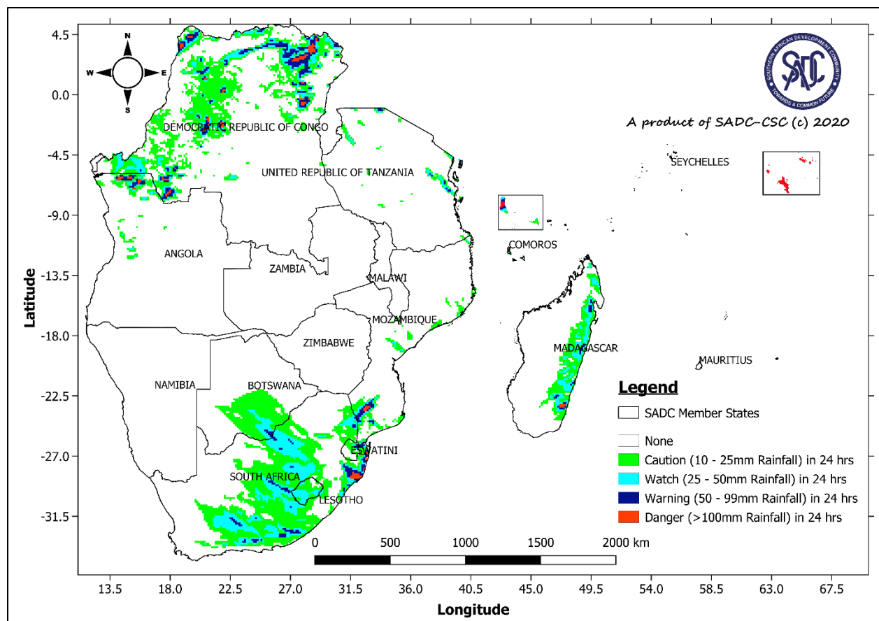
Figure 1: SADC Region's heavy rainfall advisory for the period 26 April to 02 May 2020 (Source: SADC-CSC-WRF GFS Model)
